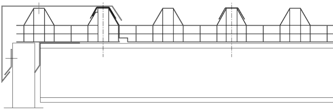
Detail corner
