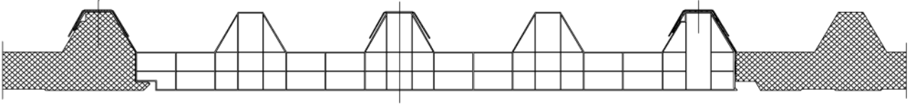
Combination glazing element with alu sandwich element
