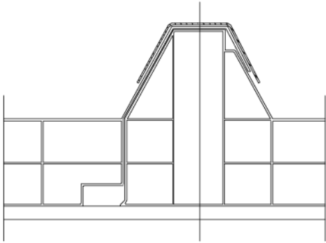
Combination glazing element with alu sandwich element
