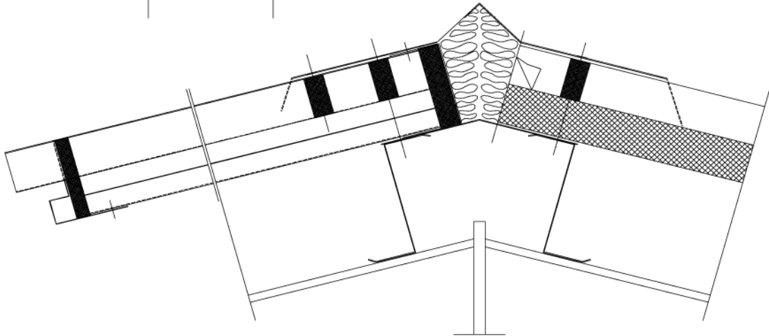
Detail peak
